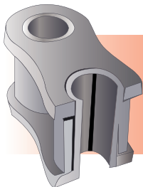
CONVENTIONAL SPLIT BUSHING ROLLER CHAINS
